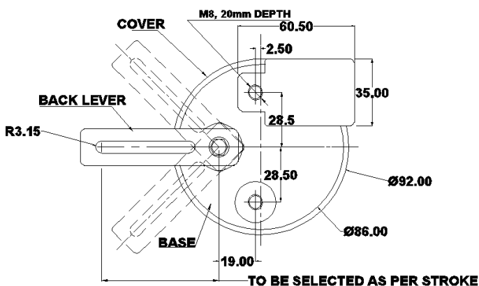
Mounting details with dimensions
