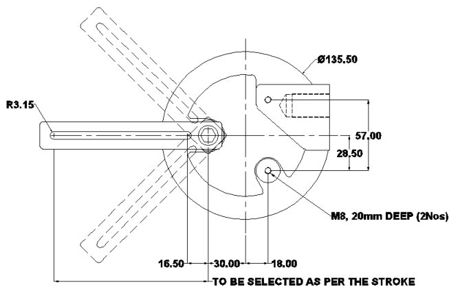
Mounting details with dimensions
