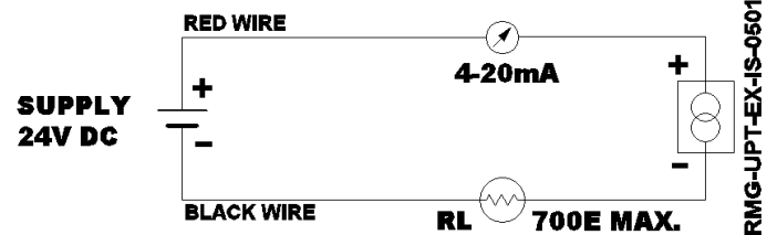
Connection diagram
