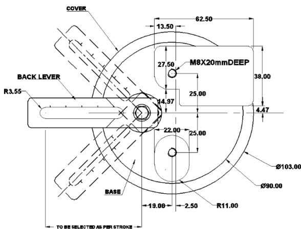
Mounting details with dimensions
